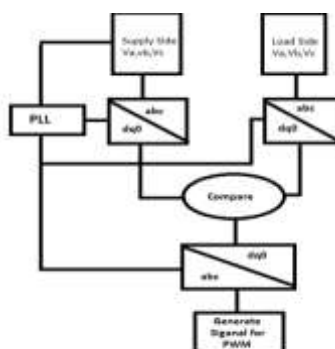
Figure-4: Control Block of DVR
