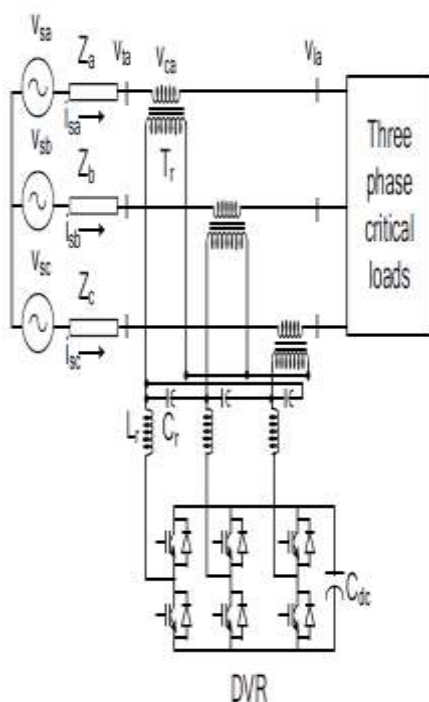
Figure-2 (a) Schematic diagram of DVR
